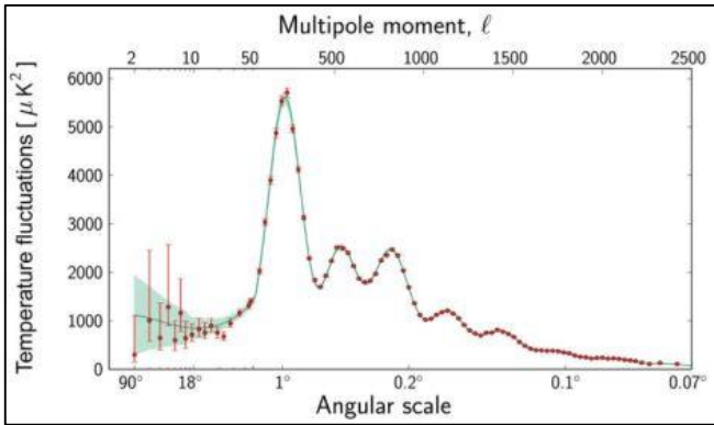
Figure 2. Planck's power spectrum of temperature fluctuations in the cosmic microwave background. The fluctuations are shown at different angular scales on the sky. Red dots with error bars are the Planck data. The green curve represents the standard model of cosmology, \Lambda CDM. The peak at 1 degree is consistent with a flat geometry of the universe, the height of the second peak with 5%, and the second and third peaks with 26% dark matter (2).
