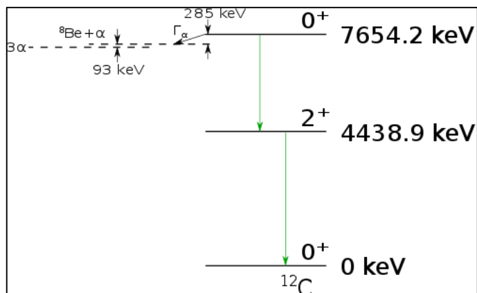
Figure. 1. Shows the first two excited states of C-12.
