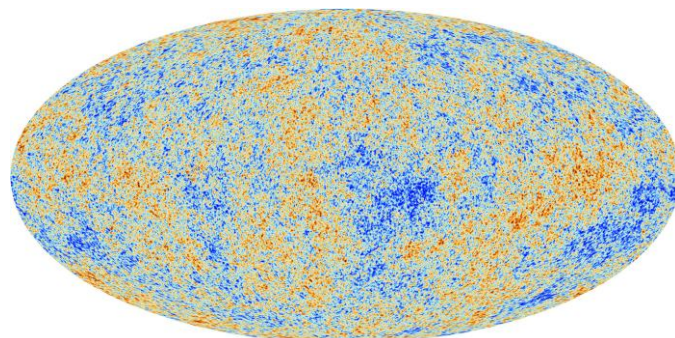
Figure. 1. Cosmic microwave background seen by Planck system.
